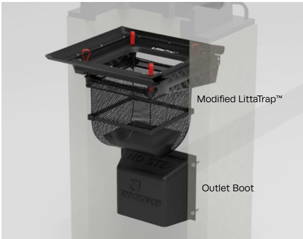
EnviroBasin™ Components
