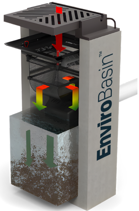
EnviroBasin™ Standard Grate Inlet
